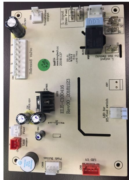
Main PCB, New Style
