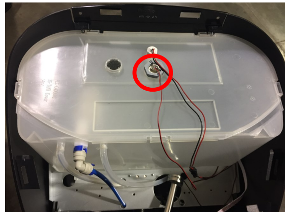
Reservoir Lid & UV, New Style
